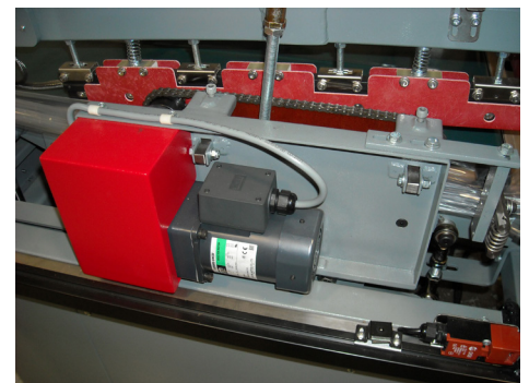
Positive Drive Film Feed (Feeds thin gauge films)
